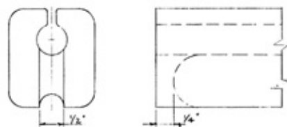
DETAIL OF BOOM AT OUTHAUL SCALE - FULL SIZE
